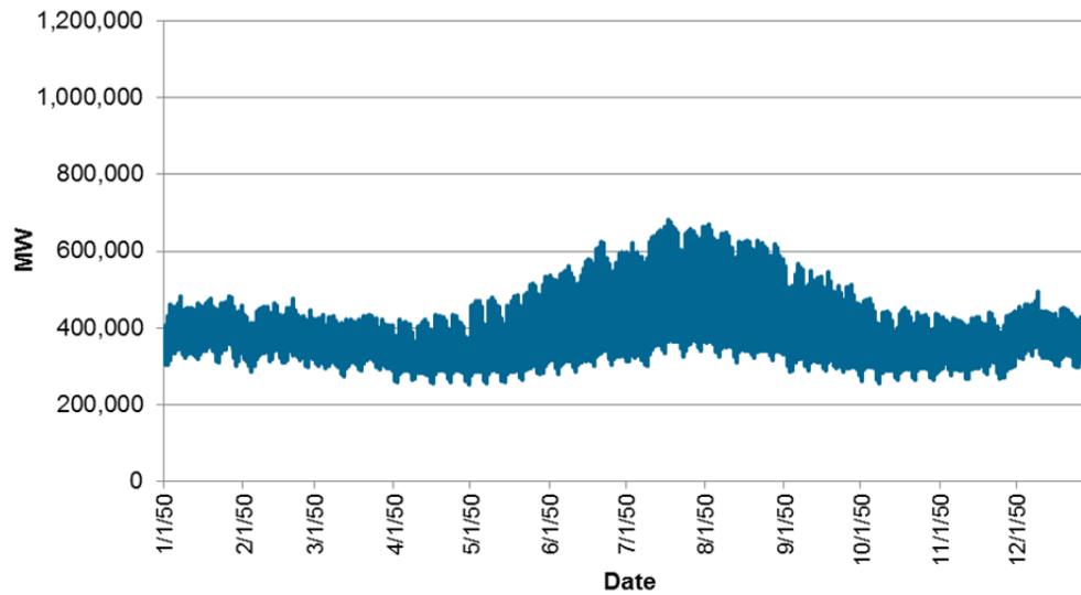
Figure 3. Non-PEV Low-Demand hourly load profile, 2050.
