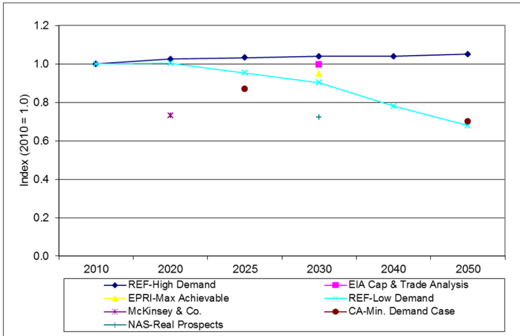
Figure 8. Comparison of commercial electricity intensities from various studies.
