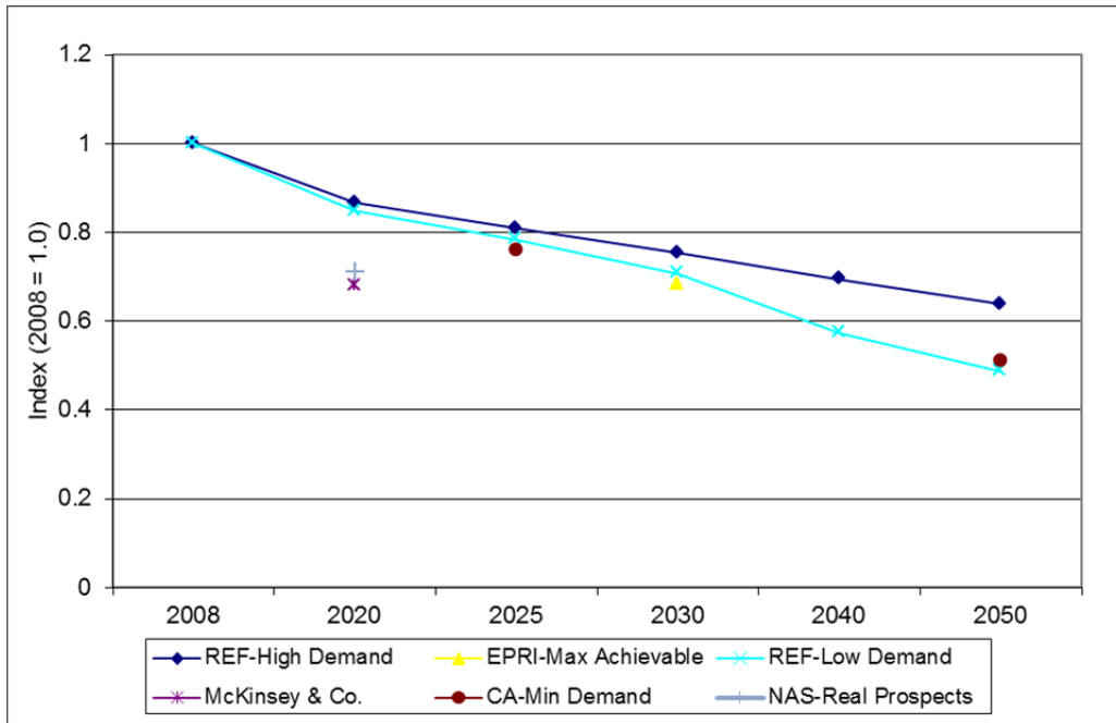
Figure 9. Comparison of industrial electricity intensities from various studies.
