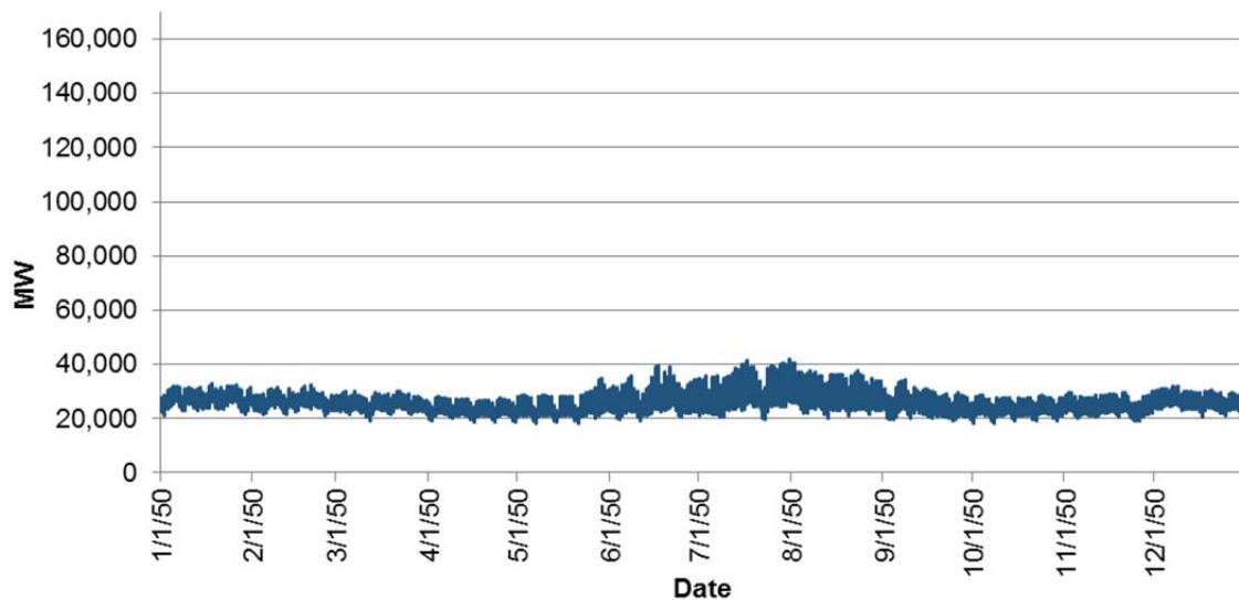
Figure 5. Non-PEV Hourly Demand in 2050, Region 4 (Mid-America Interconnected Network).
