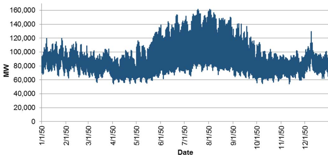
Figure 6. Non-PEV Hourly Demand in 2050, Region 9 (Southeastern Electric Reliability Council).
