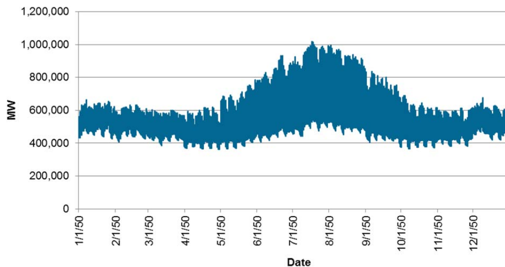
Figure 2. Non-PEV High-Demand hourly load profile, 2050.
