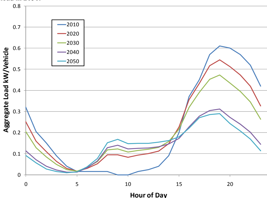
Figure 4. Shape and transition of fixed hourly aggregate load profile for PEVs.
